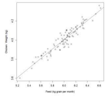
Linear Model (a straight line): y = b_0 + b_1x_1 + error
